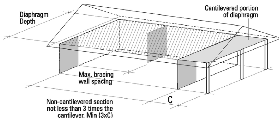
Figure 6 Cantilevered Diaphragms
