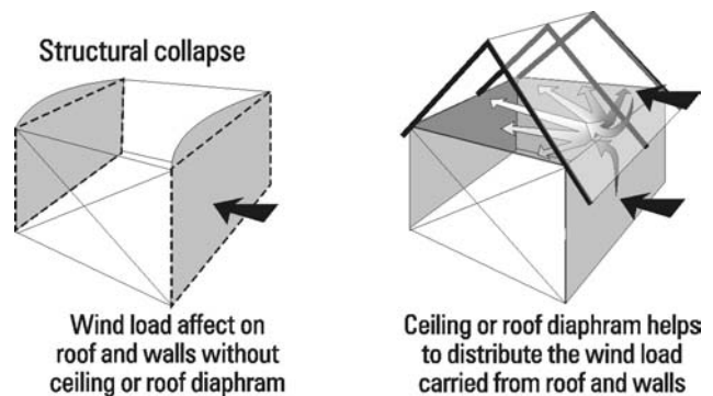
Figure 2 Horizontal Diaphragms
