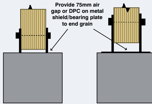
Figure 6.2: Isolation of timber from moisture traps.
