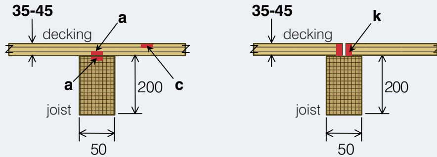
Figure 5.5: Typical dimensions of commercial decking and locations of interest for service lives.
