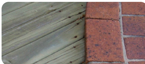
Corrosion of HDG nails close to pool edge.
