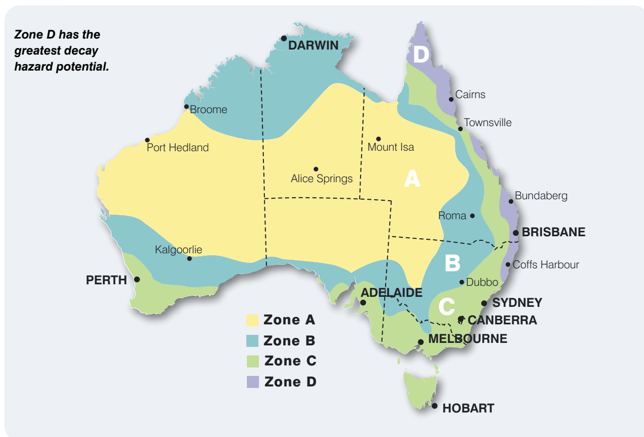
Figure 5.2: Above ground decay hazard zones for Australia.
