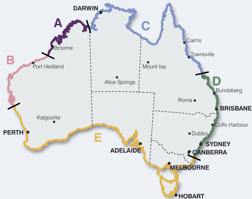
Figure 8.4: Coastal zones related to corrosion due to airborne salt.
