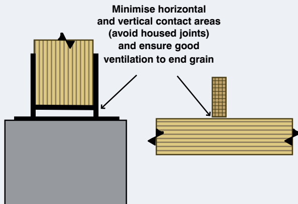
Figure 6.3: Moisture traps.
