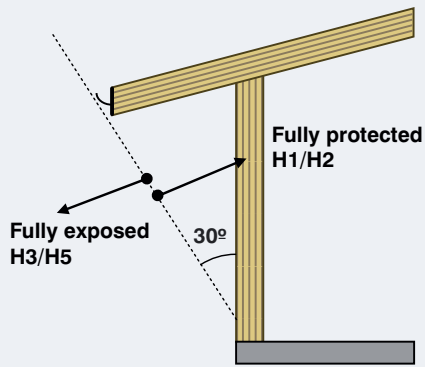
Figure 6.1: Architectural detailing – shielding.
