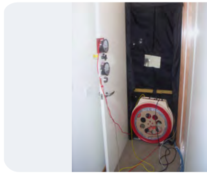
Figure 28: Blower door testing.
