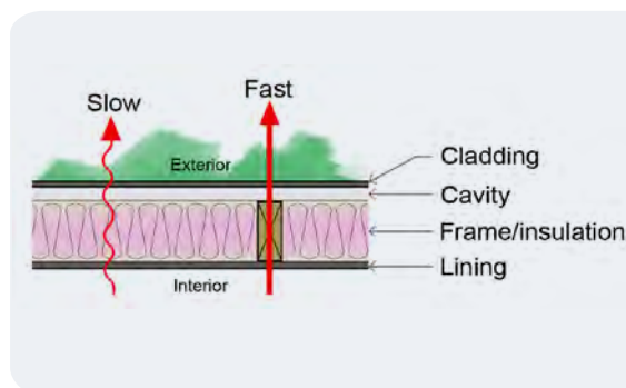
Figure 31: Avoiding conducted heat loss.
