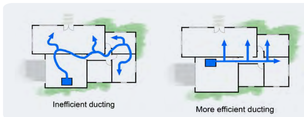
Figure 71: Duct runs. Straight duct runs improve efficiency.
