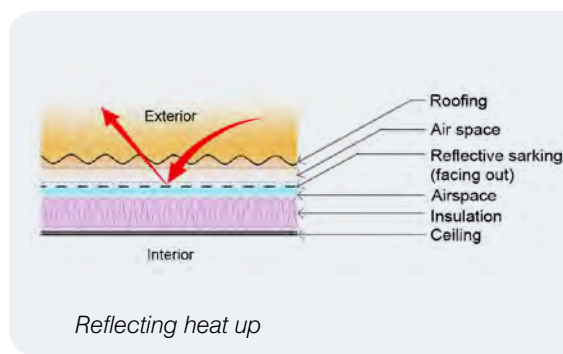
Figure 33: Diagram of reflective insulation.
