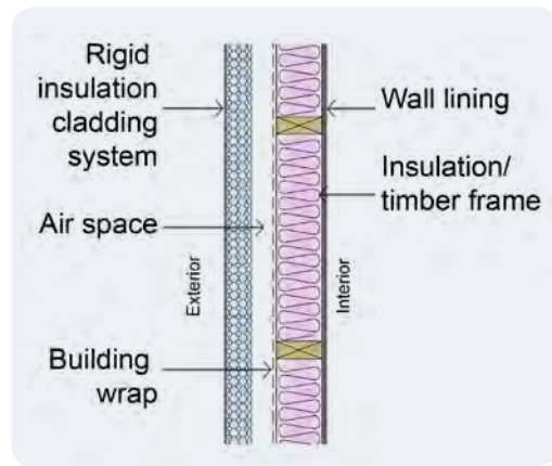
Figure 51: Over-cladding as external cladding. A still air cavity and wall wrap between the over-cladding and frame enhance insulation.
