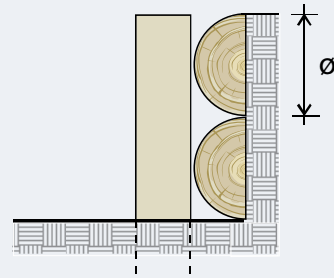
Figure 3.2 (h): Split wales (SWD)
