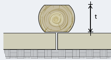
Figure 3.2 (a): Sleeper posts (HWD & SWD)
